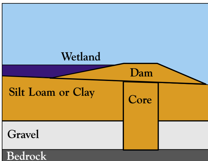
The core prevents water from leaking under the dam.
